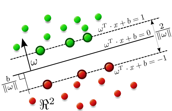
Figure 4. Schematic representation of an SVM. Red and green samples represent class zero and one respectively. Expression \|\omega\|^{-1} is the margin to each class. Samples with bold lining are support vectors. Image after. 14
